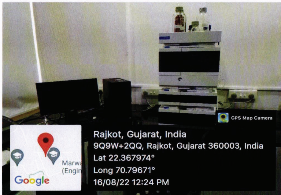
HPLC System with PDA detector, AGILENT, 1260 INFINITY
